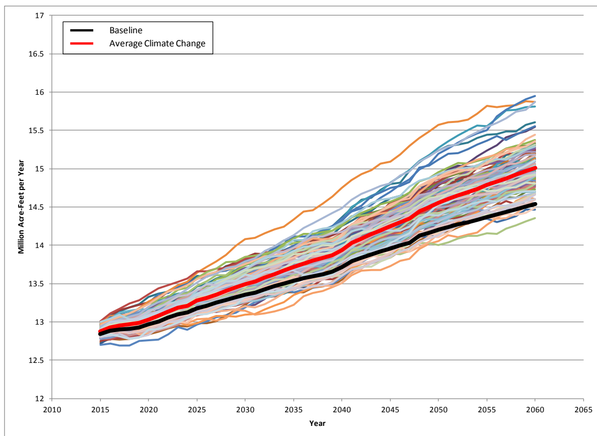
FIGURE C-21 Current Projected (A) Scenario Demands Adjusted for Future Climate Change
