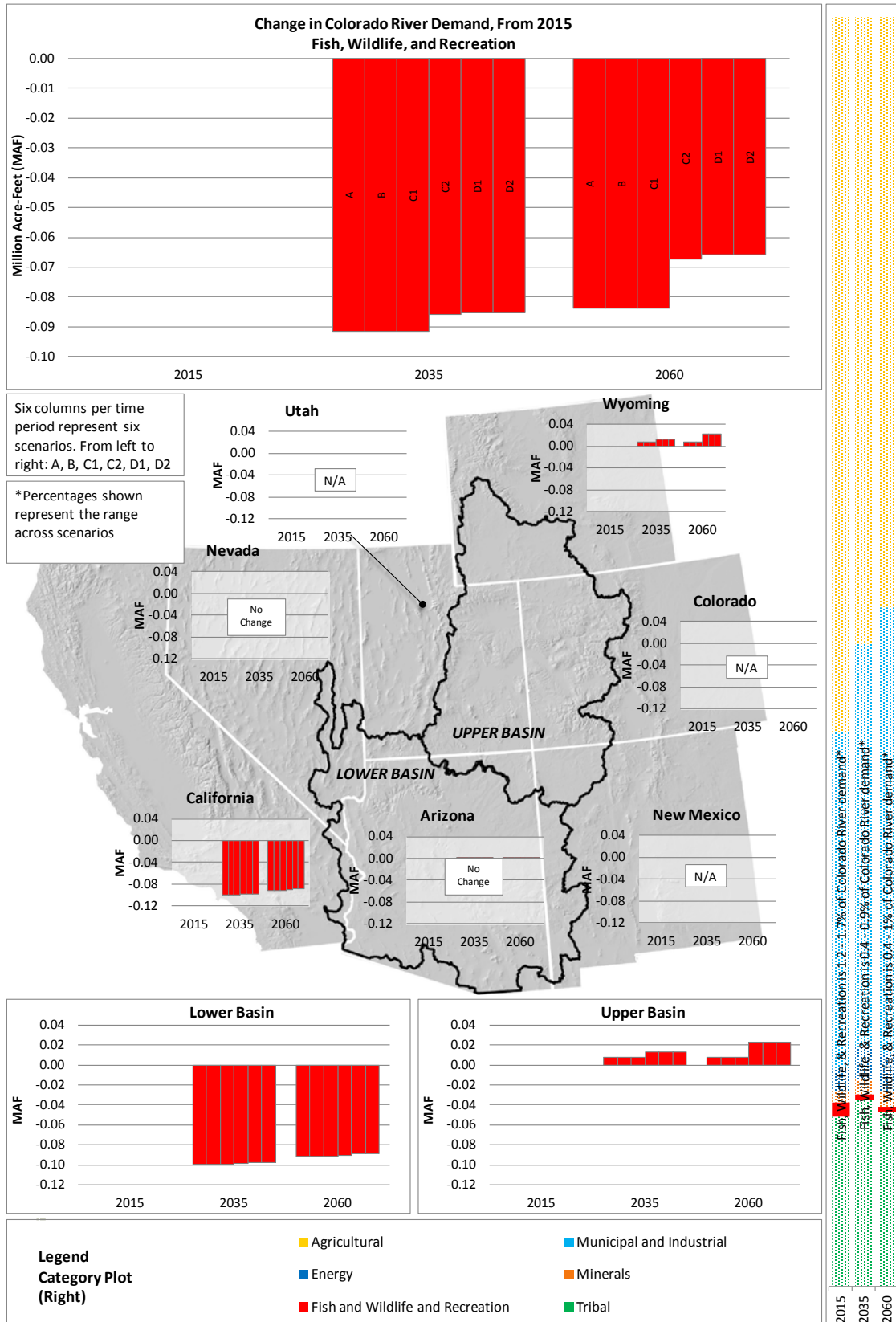
FIGURE C-16 Change in Colorado River Water Demand for Fish, Wildlife, and Recreation
