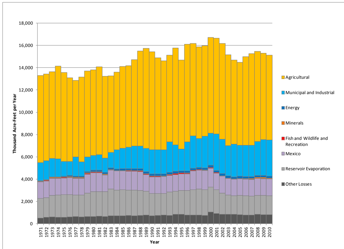
FIGURE C-4 Historical Colorado River Water Consumptive Use 1 , Delivery to Mexico, Reservoir Evaporation, and Other Losses 2 , 1971–2010
