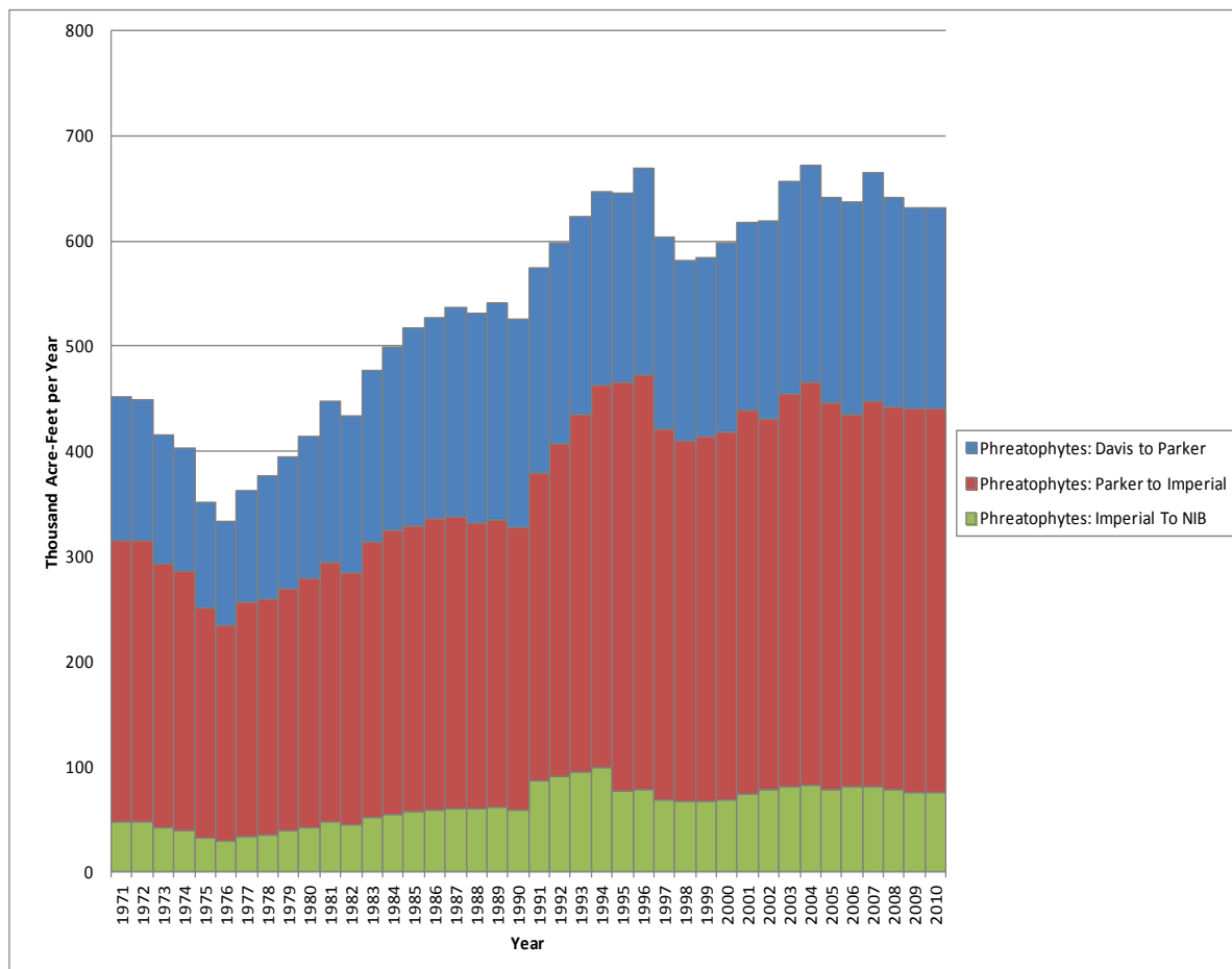
FIGURE C-20 Historical Lower Basin Phreatophyte Use, 1971–2010
