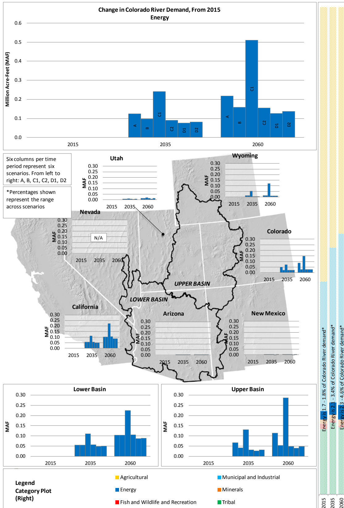
FIGURE C-14 Change in Colorado River Water Demand for Energy
