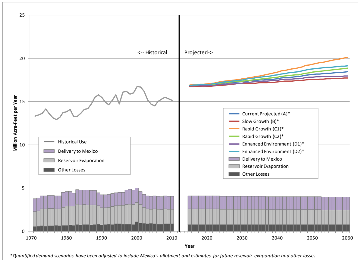
FIGURE C-8 Colorado River Basin Historical Use 1 and Future Projected Demand 1 , Delivery to Mexico 2 , Reservoir Evaporation 3 , and Other Losses 4
