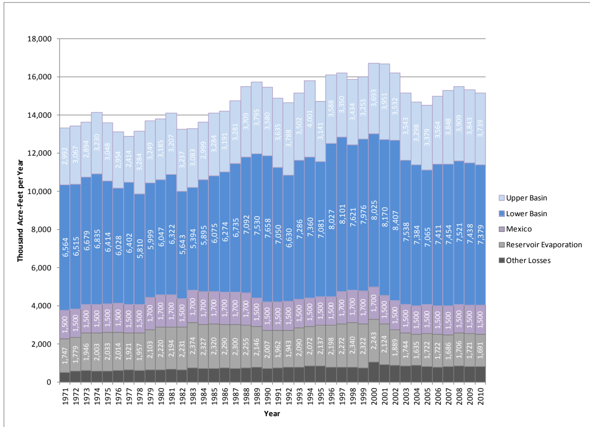
FIGURE C-3 Historical Colorado River Water Consumptive Use 1 and Loss by Basin, Mexico, Reservoir Evaporation 2 , and Other Losses 3 , 1971–2010
