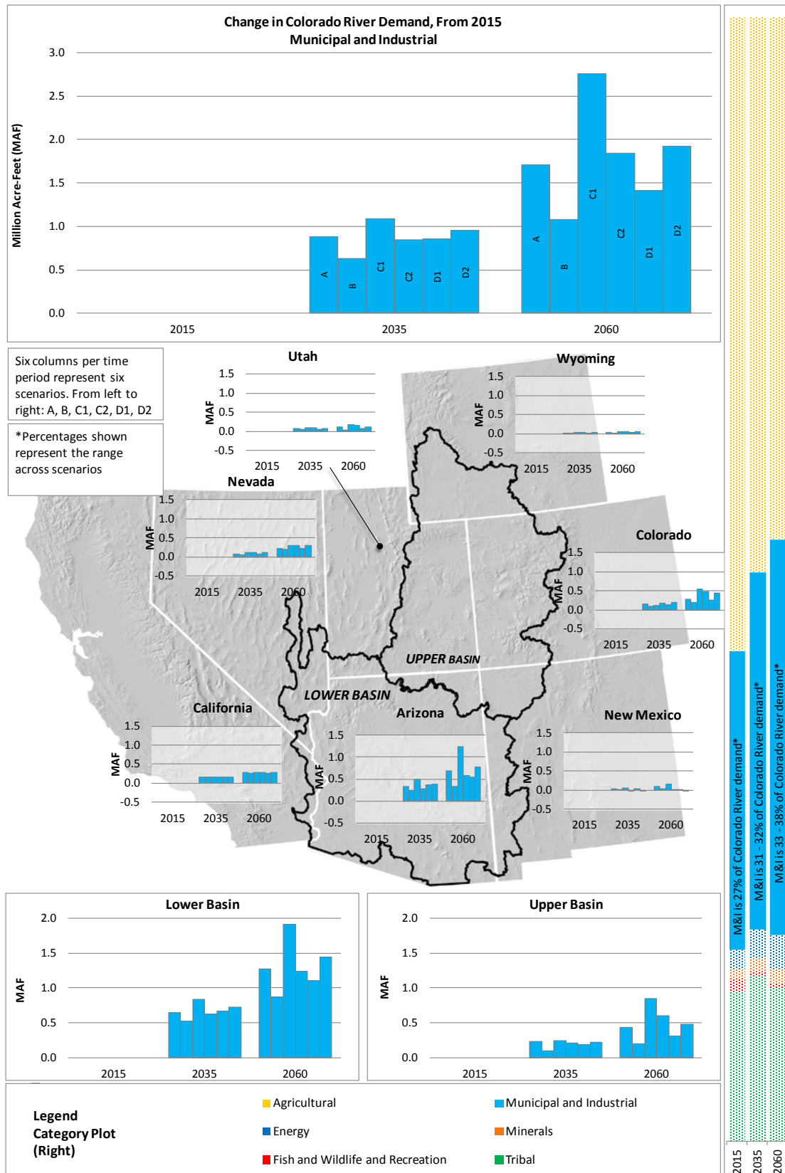
FIGURE C-13 Change in Colorado River Water Demand for Municipal and Industrial
