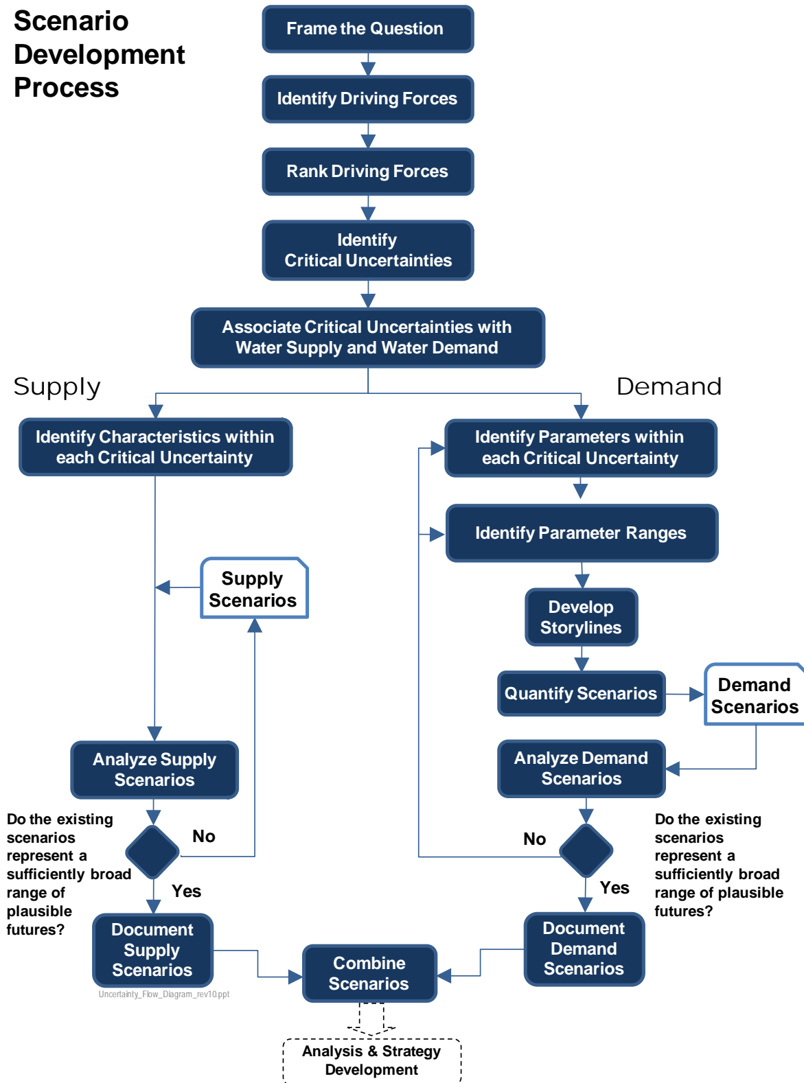
FIGURE C-5 Scenario Development Process
