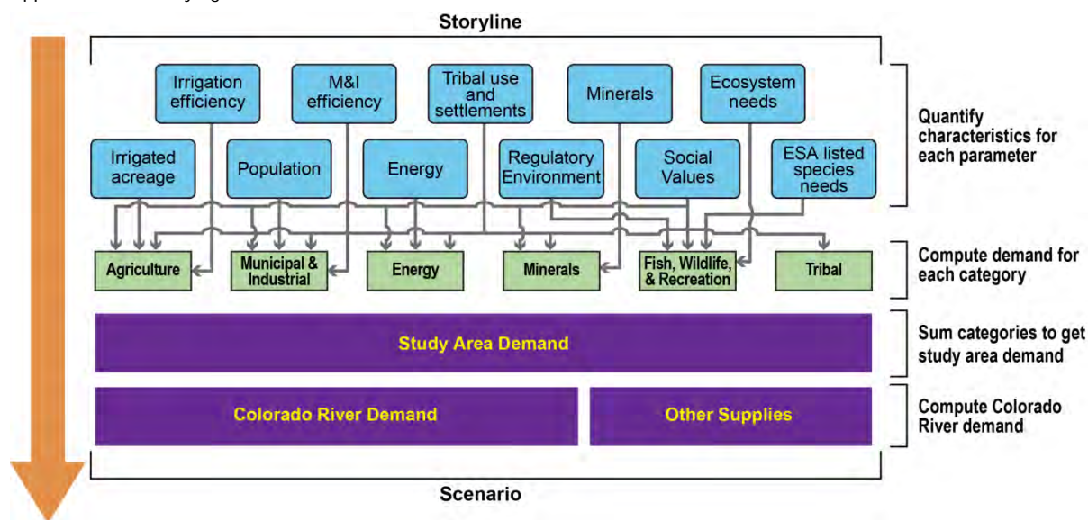
FIGURE C-6 Approach to Quantifying Demand Scenarios 1
