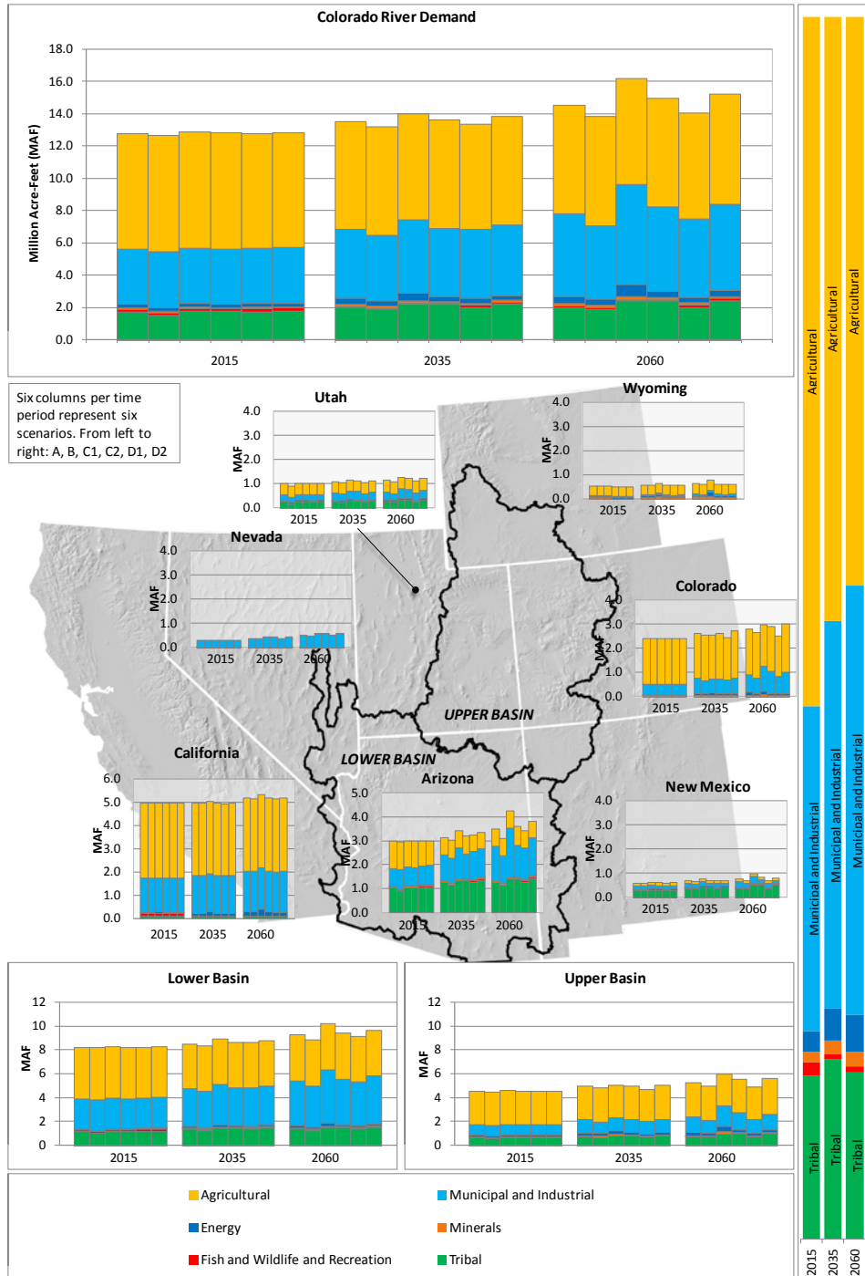
FIGURE C-10 Colorado River Water Demand by Category 1,2
