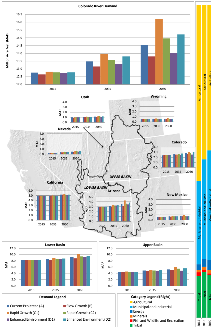
FIGURE C-9 Colorado River Water Demand 1,2
