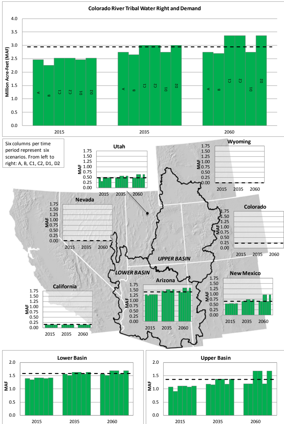
FIGURE C-18 Colorado River Basin Tribal Diversion Rights (dotted line) and Diversion-Based Demand 1,2,3
