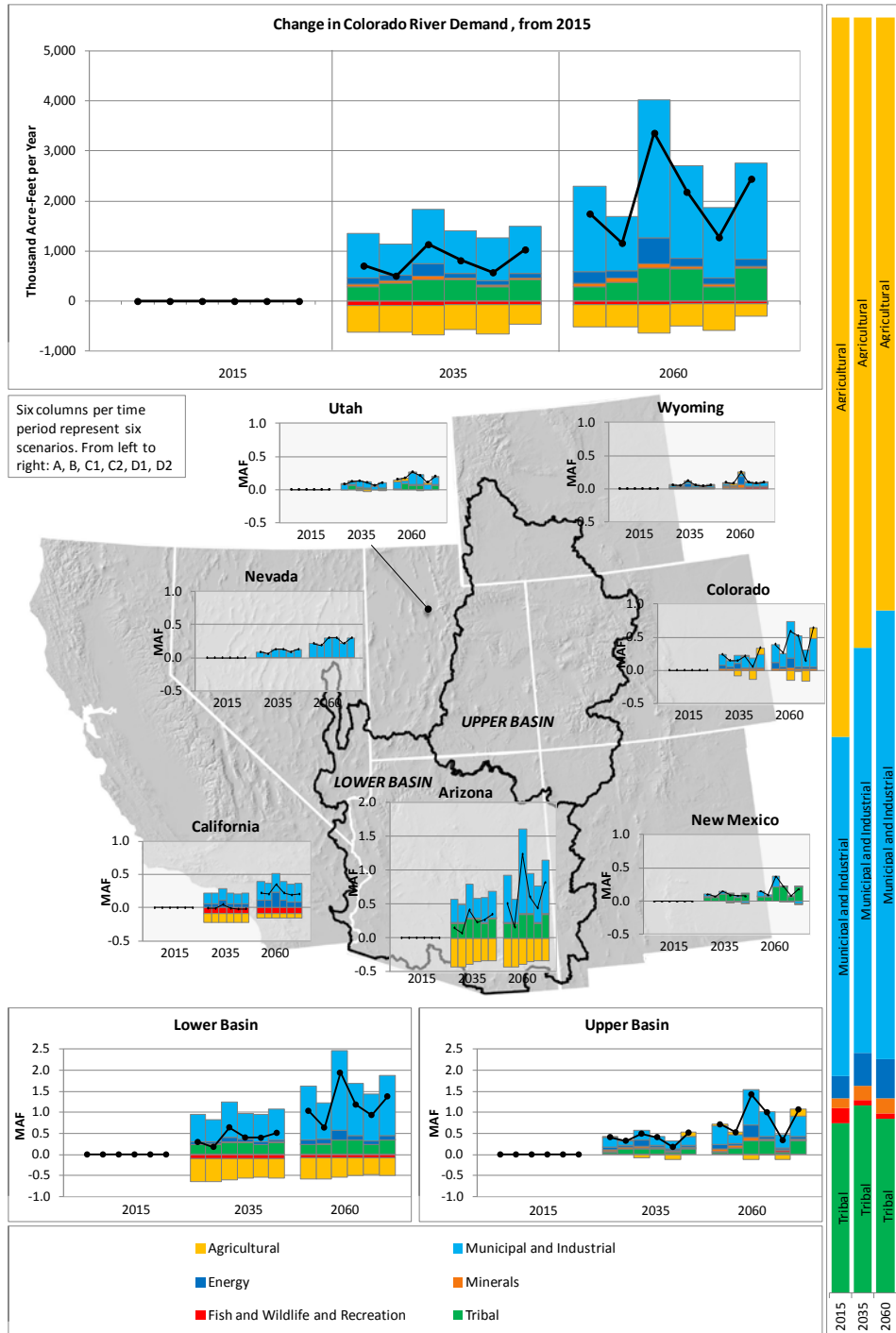
FIGURE C-11 Change in Colorado River Water Demand from 2015 by Category 1,2
