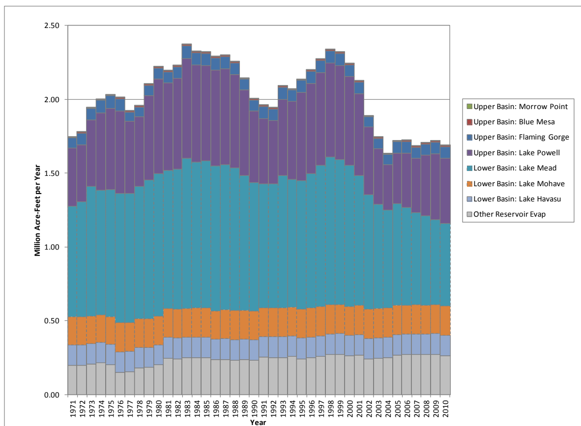
FIGURE C-19 Reservoir Evaporative Losses
